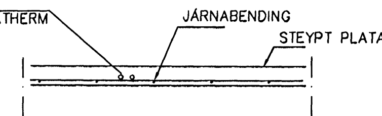
LAGNIR, SNID, 1:20
