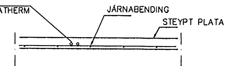
LAGNIR, SNID, 1:20
