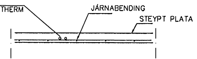
LAGNIR, SNID, 1:20
