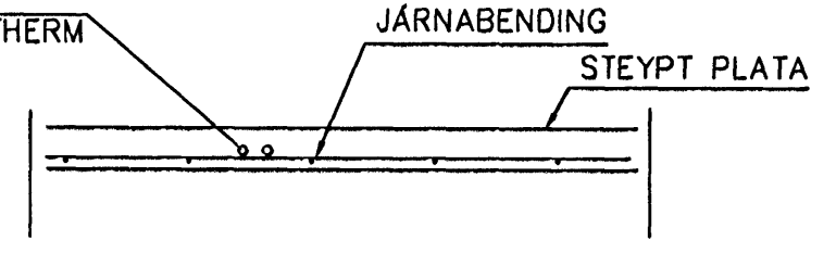
LAGNIR, SNID, 1:20
