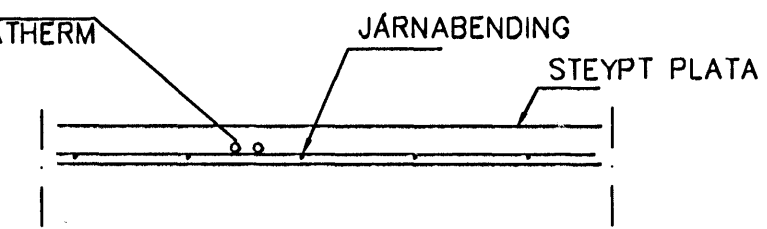
LAGNIR, SNID, 1:20
