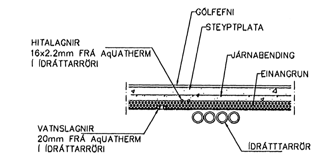
LAGNIR, SNID, 1:20
