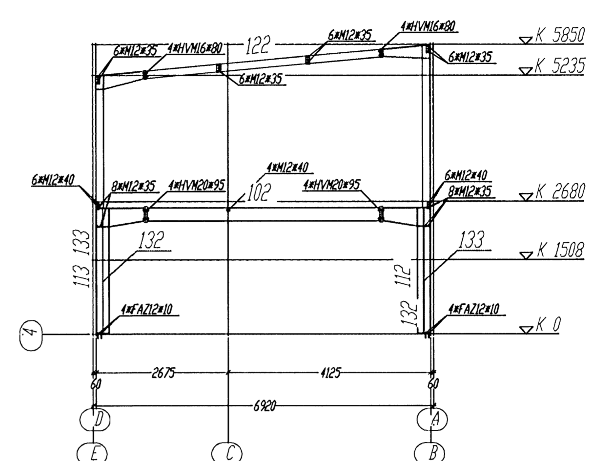
Section Axis 4 (Sc.1:75)
