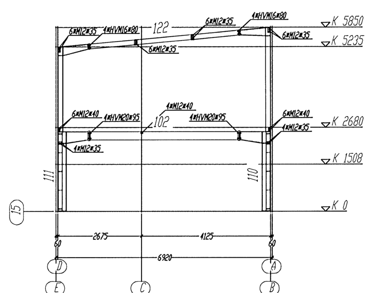
Section Axis 15 (Sc.1:75)
