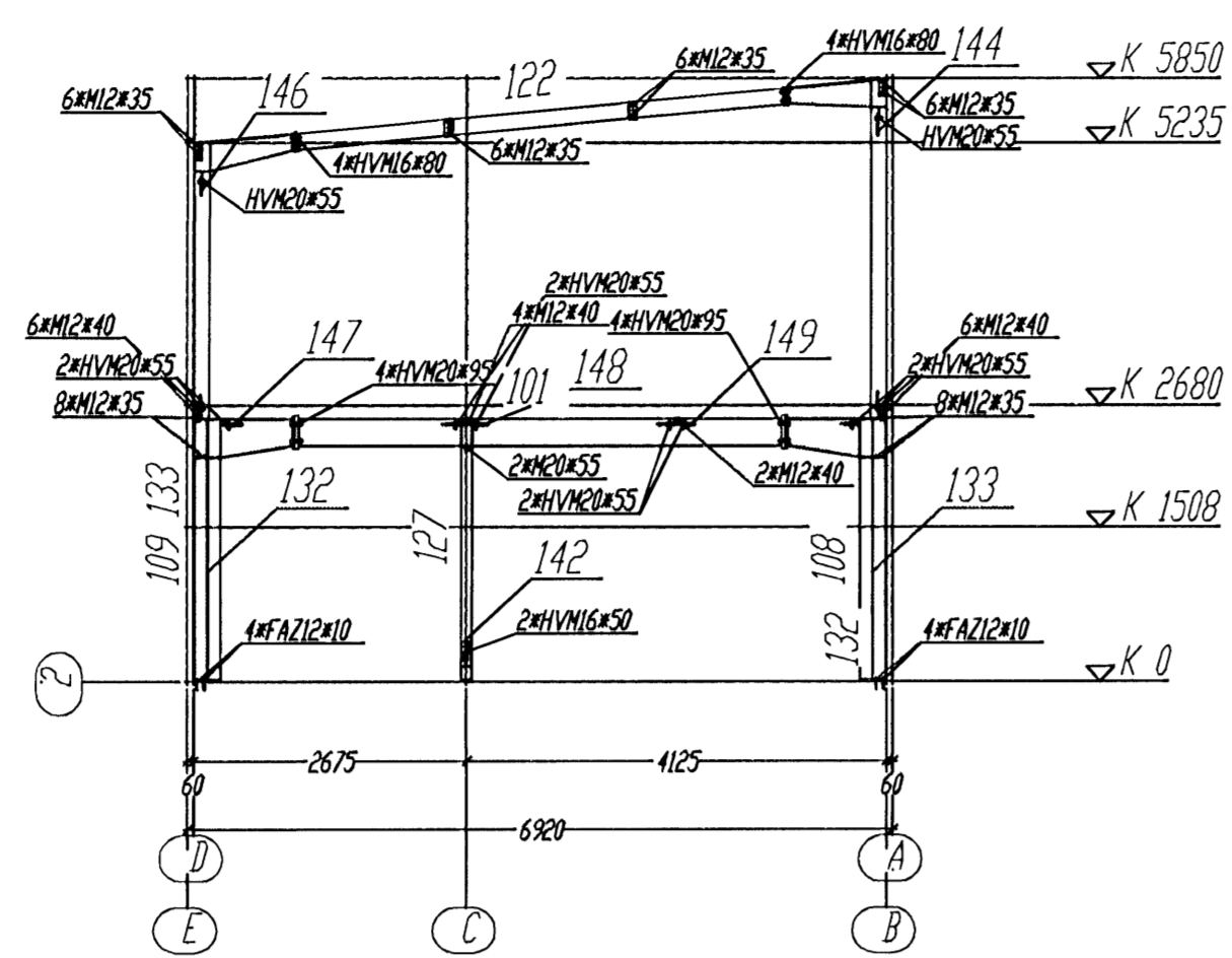
Section Axis 2 (Sc.1:75)
