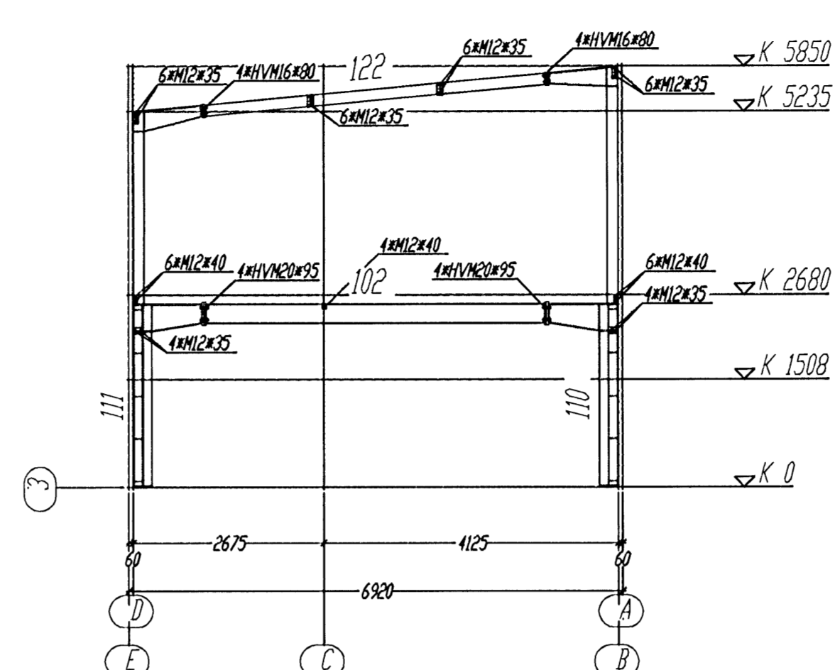
Section Axis 3 (Sc.1:75)
