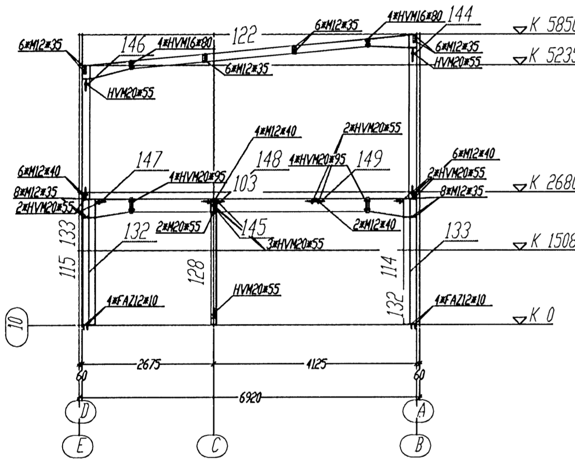
Section Axis 10 (Sc.1:75)
