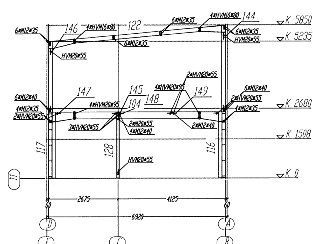
Section Axis 11 (Sc.1:75)
