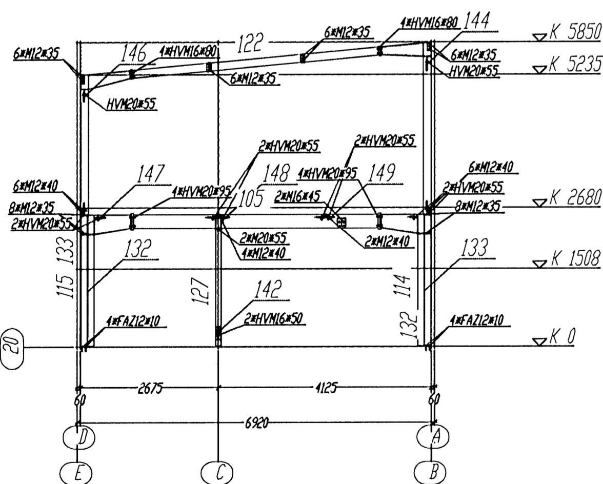
Section Axis 20 (Sc.1:75)
