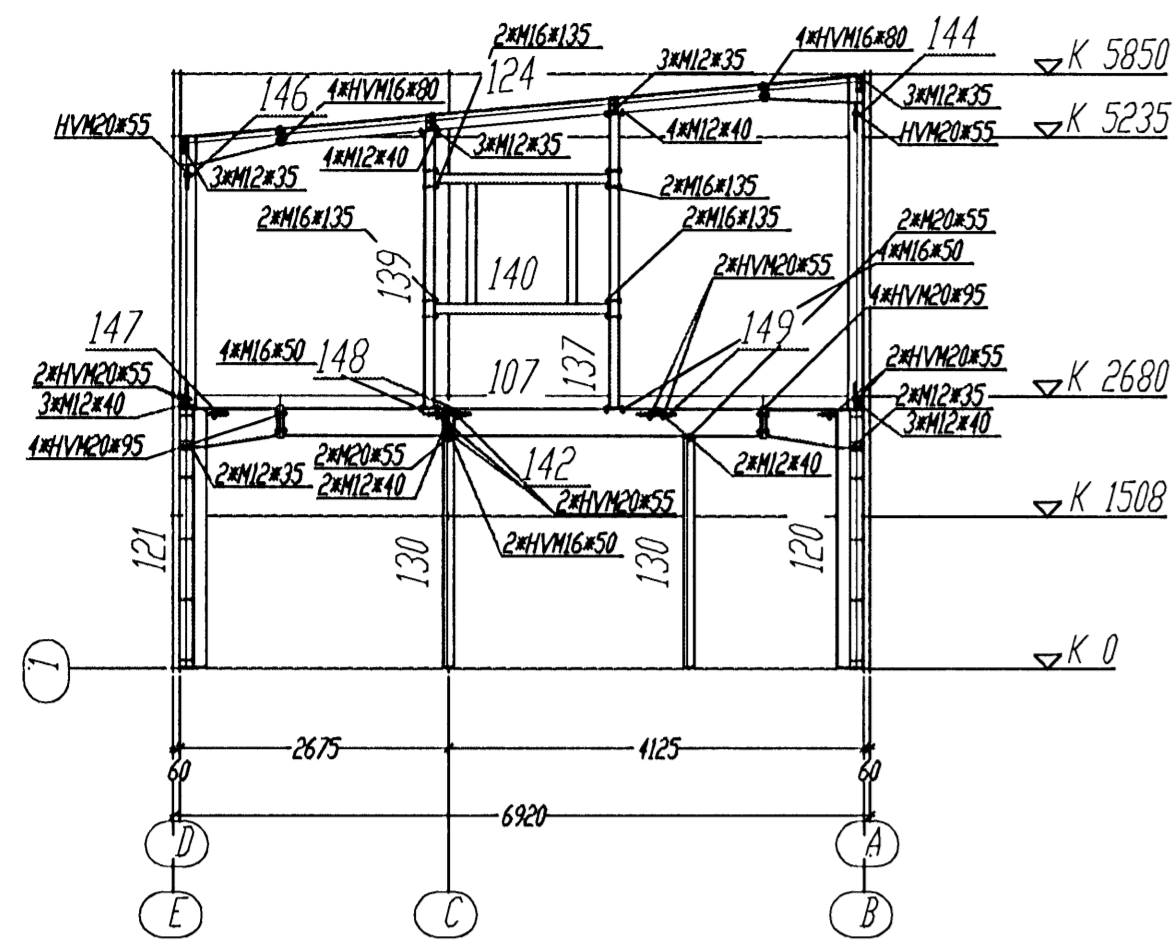
Section Axis 1 (Sc.1:75)
