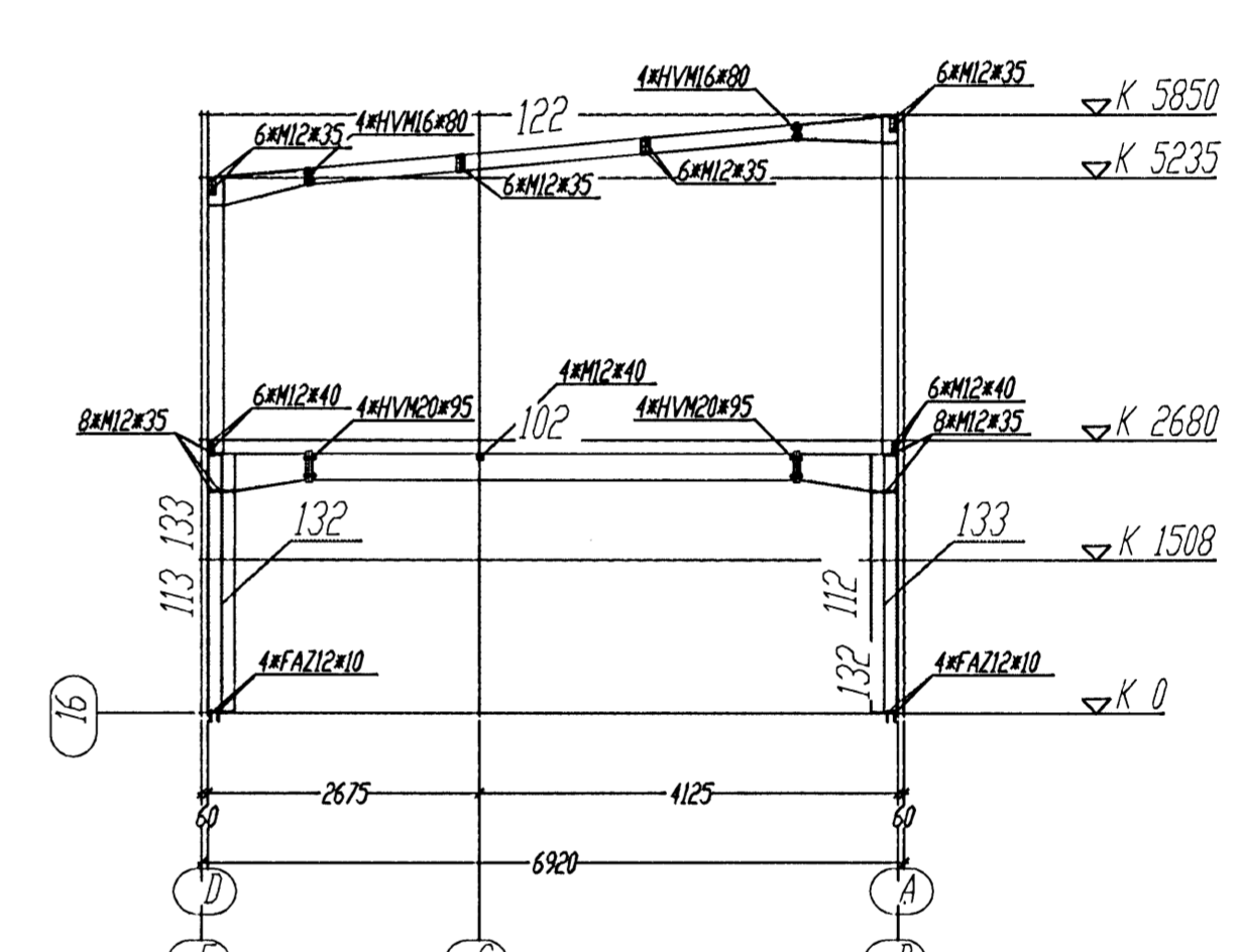
Section Axis 16 (Sc.1:75)
