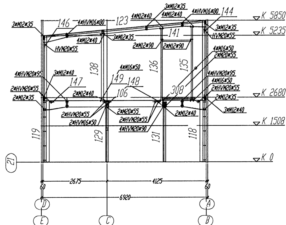
Section Axis 21 (Sc.1:75)
