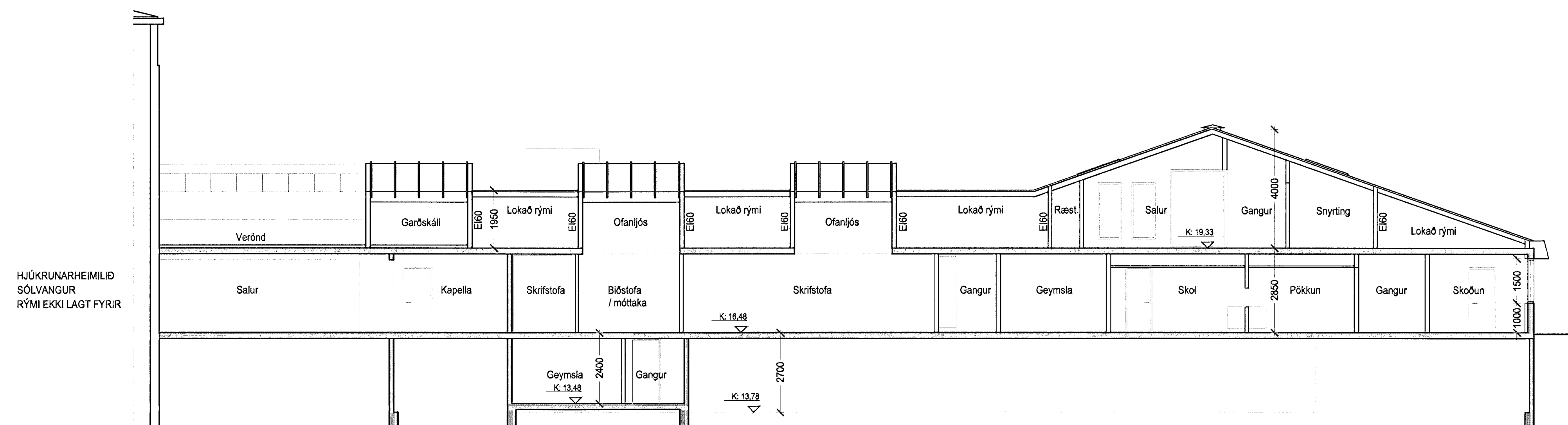
1 SNID 1:100
