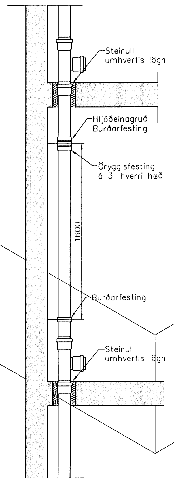
Fallþipa, festingar 1:20
