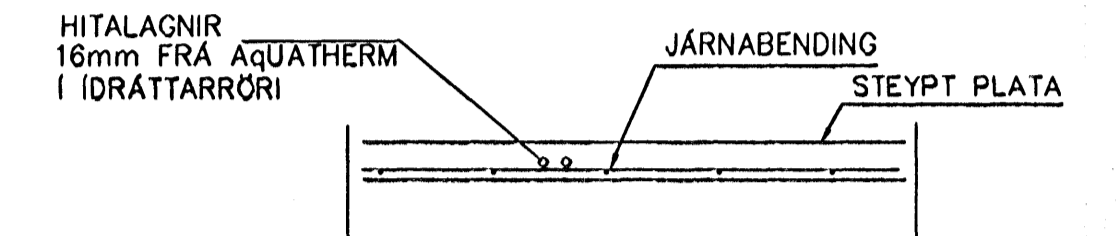
LAGNIR, SNID, 1:20
