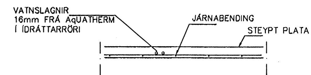
LAGNIR, SNID, 1:20
