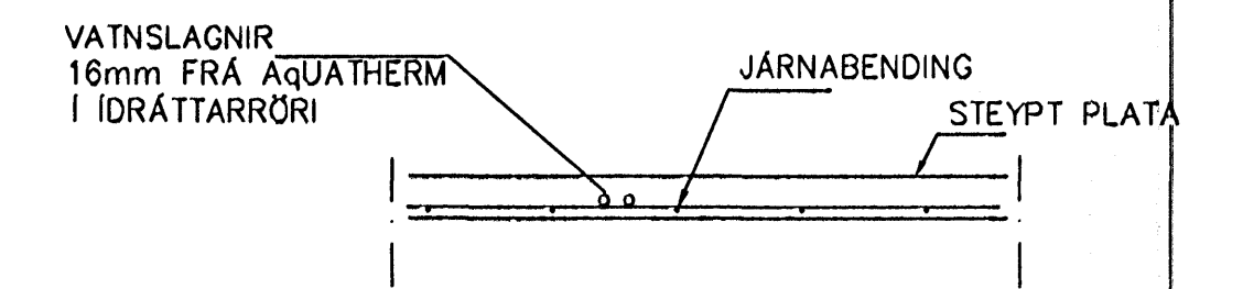
LAGNIR, SNID, 1:20
