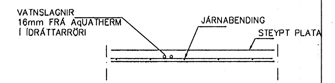
LAGNIR, SNID, 1:20
