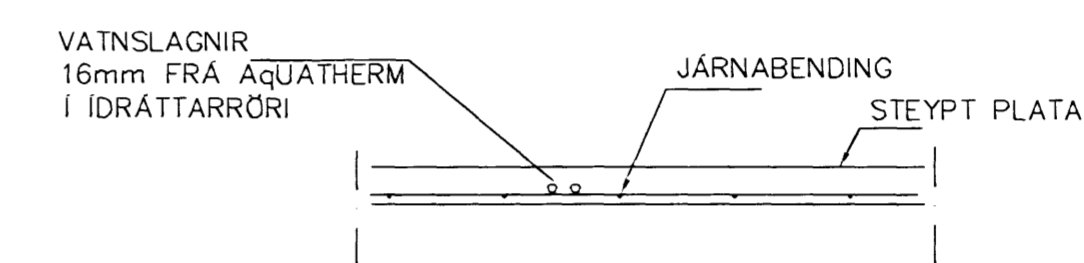
LAGNIR, SNID, 1:20
