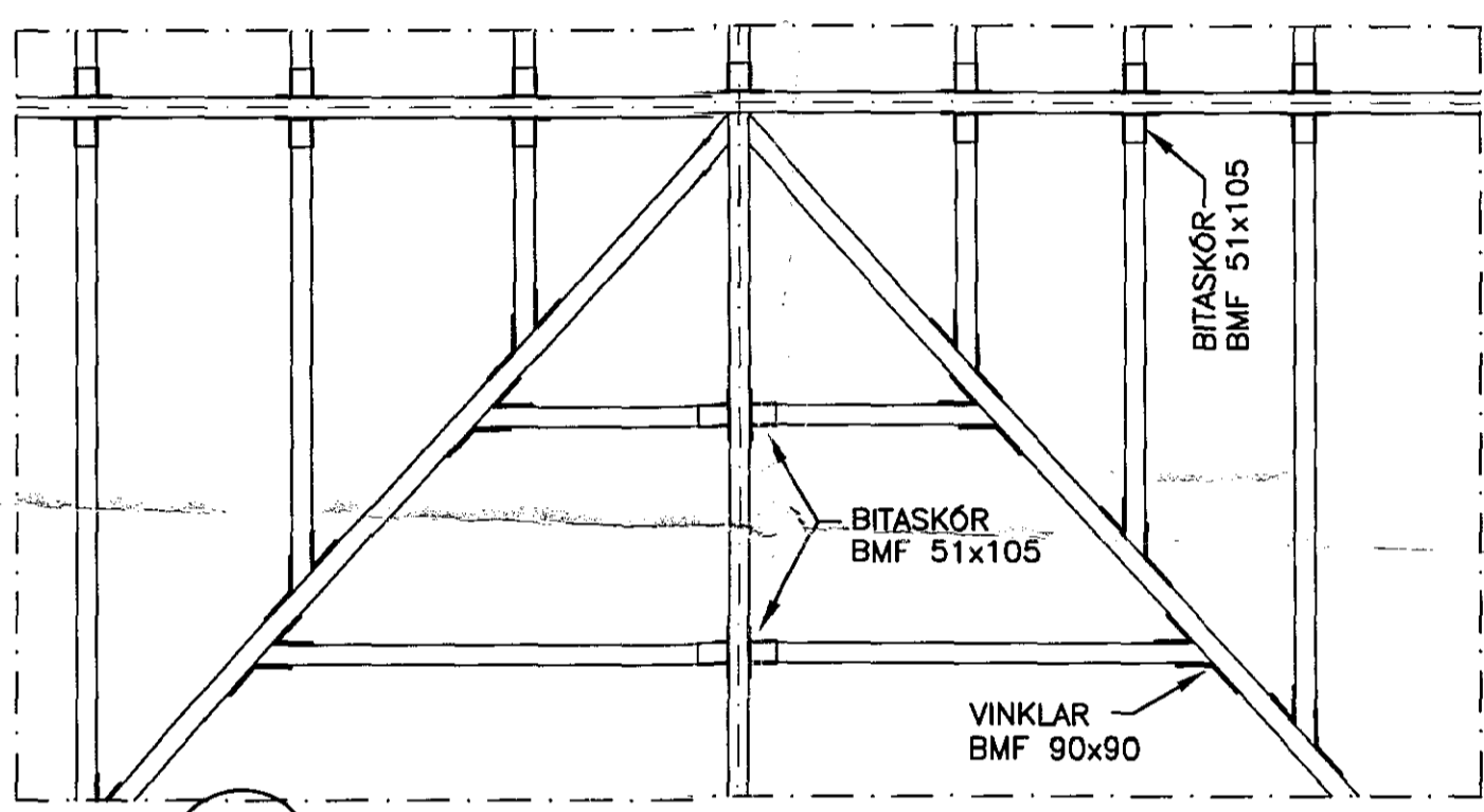
f DEILI 102/103 MKV. 3
