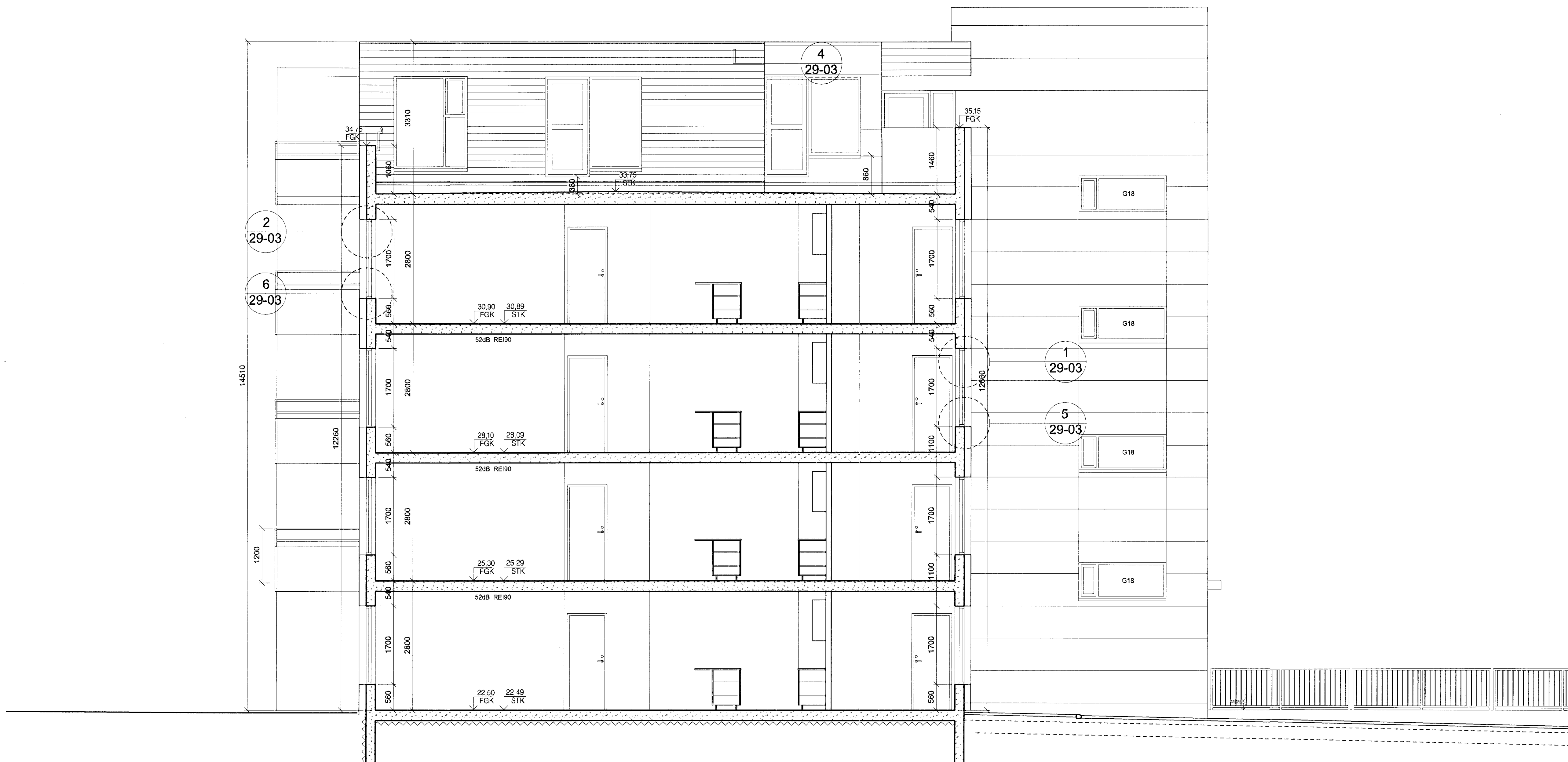
F-F 20-02 20-04 20-06 20-08 20-10 20-12 20-14 SNEIÐING 1:50
