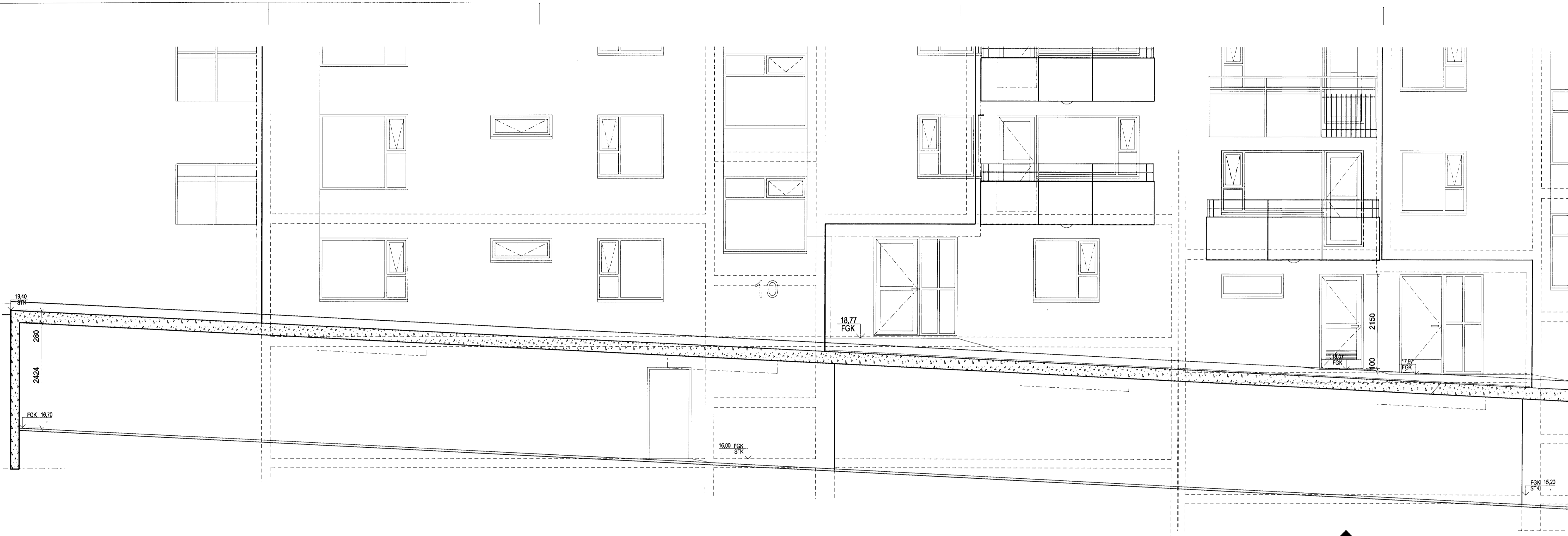
E-E 20-01 SNEIDING 1:50 Efri hluti
