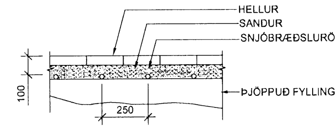
A SNID 1:20
