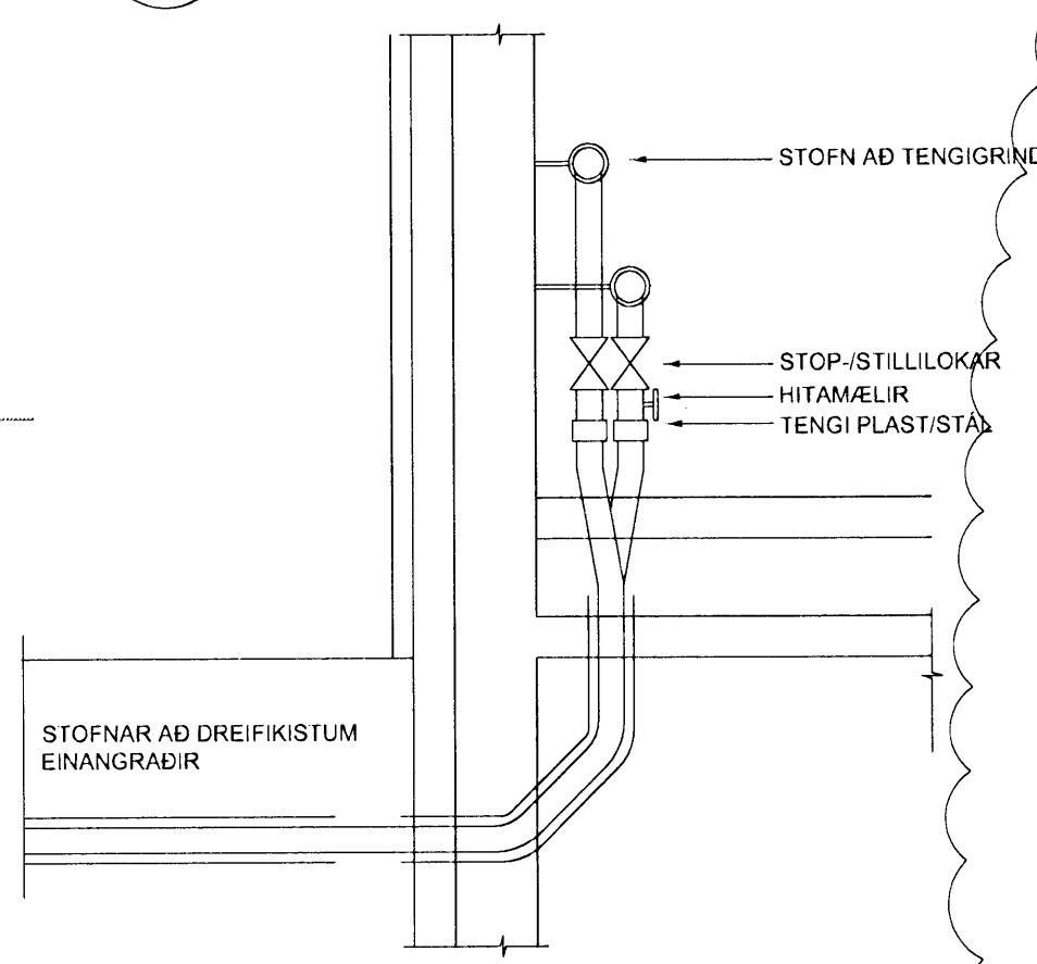
C SNID 1:20
