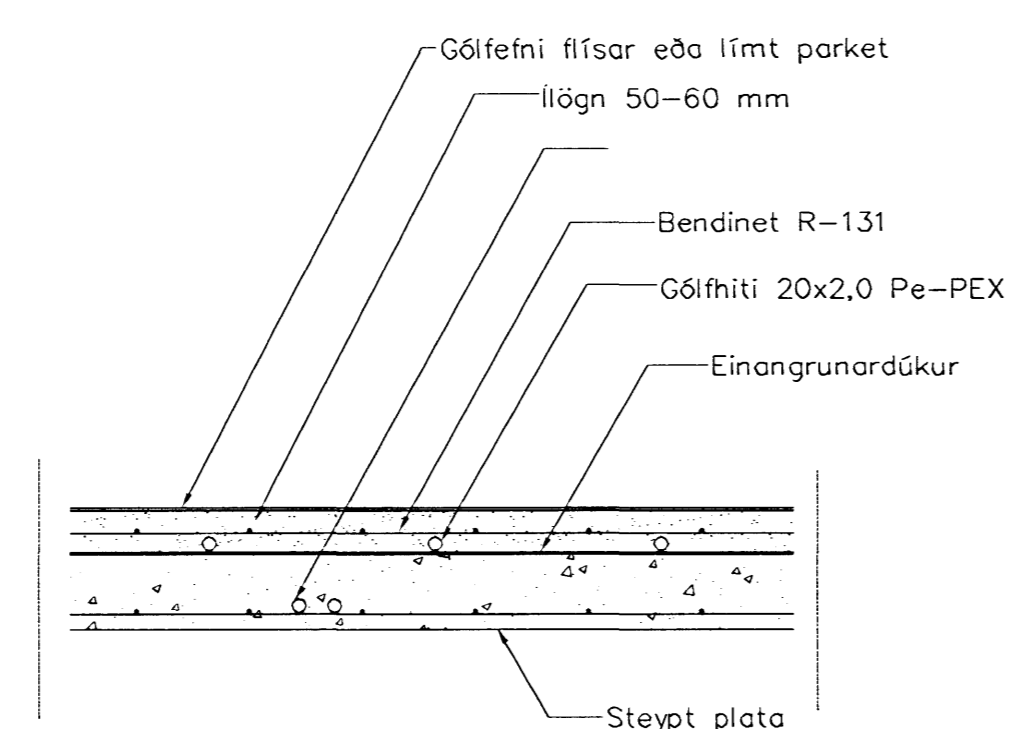
LAGNIR, SNIB, 1:20
