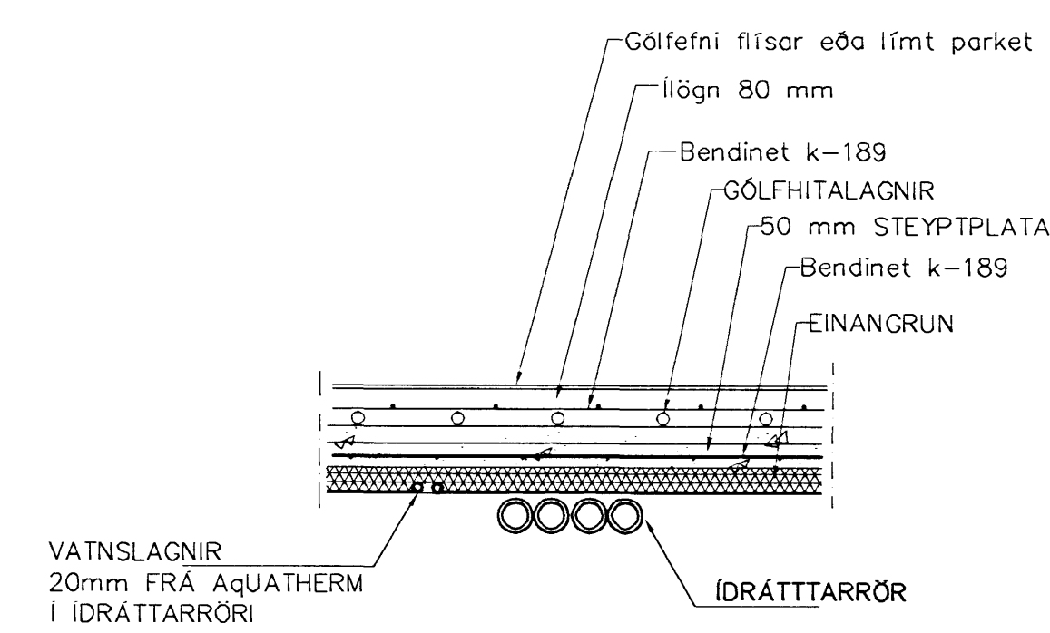
LAGNIR, SNID, 1:20
