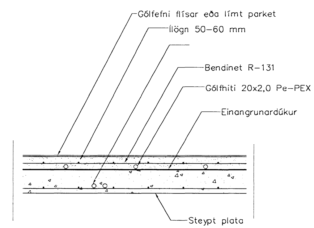
LAGNIR, SNIB, 1:20
