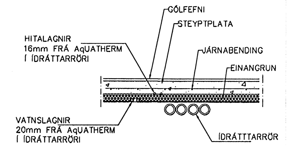
LAGNIR, SNID, 1:20
