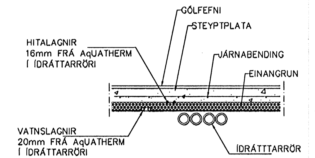
LAGNIR, SNID, 1:20
