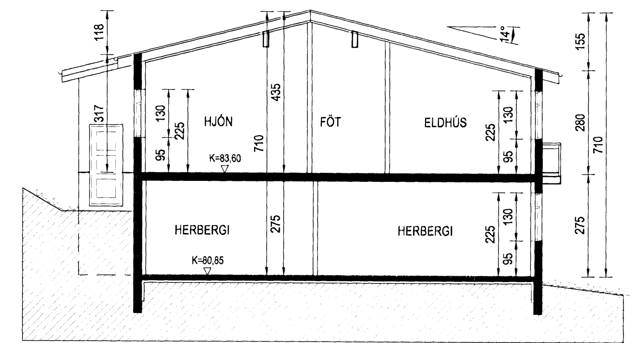
SNID B-B
