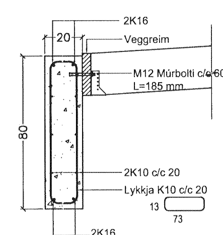
B1.1 BITI B1.1. 1:20.
