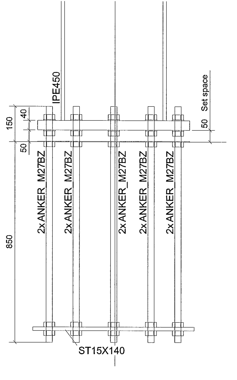
Column foot (B)
