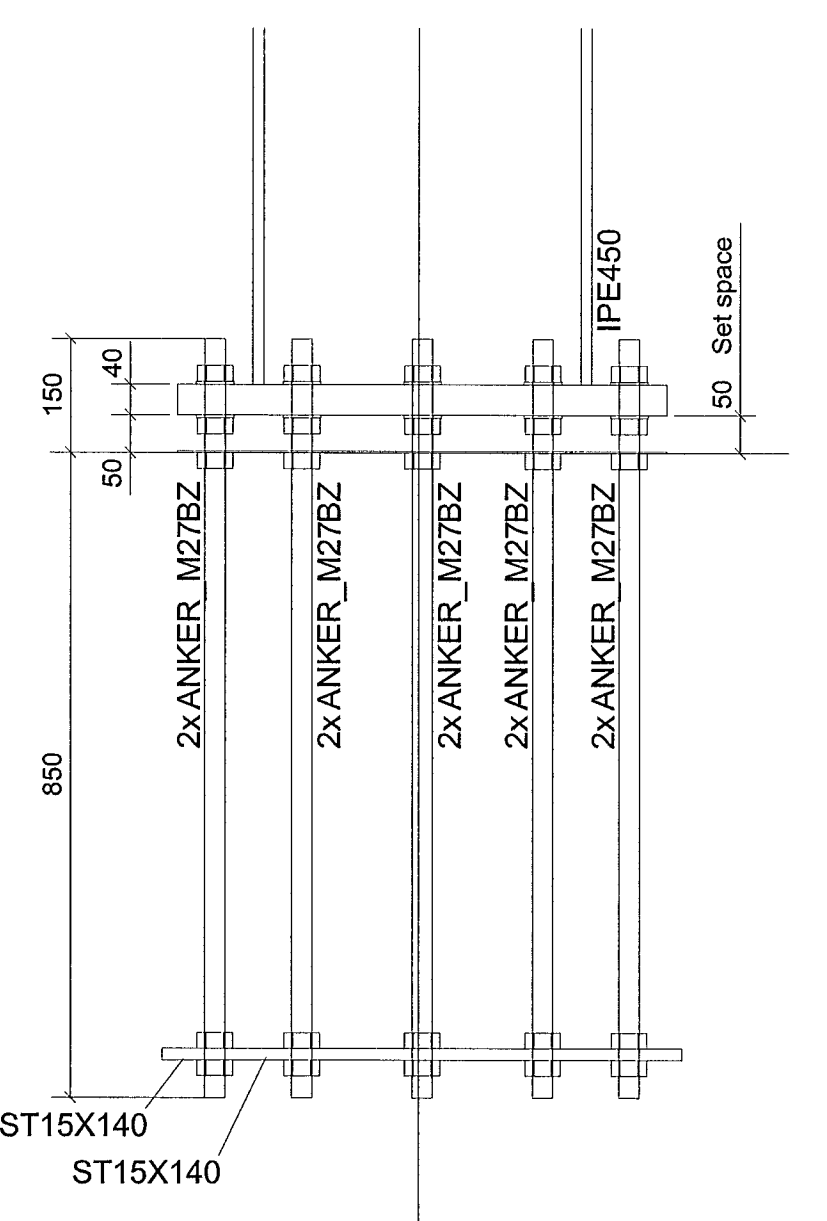
Column foot (A)
