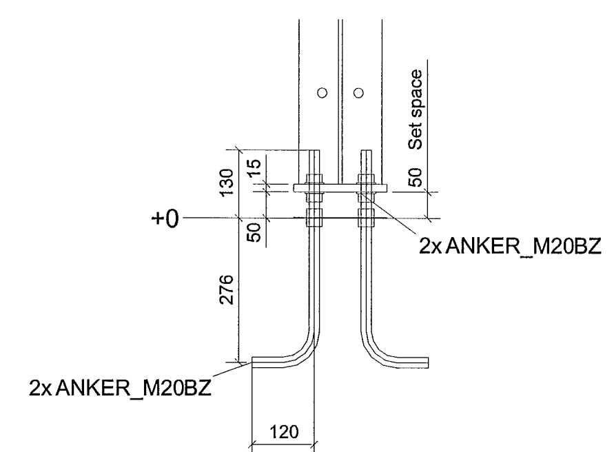
Column foot (C)
