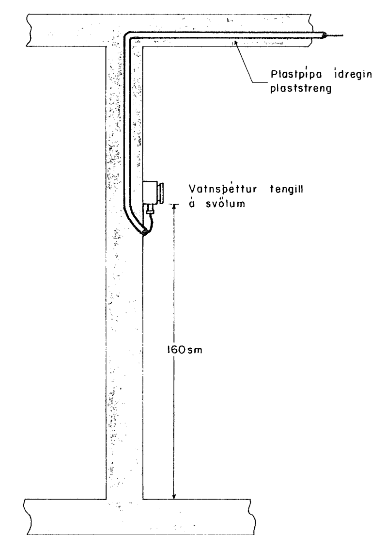
SNID C - C M = 1:20
