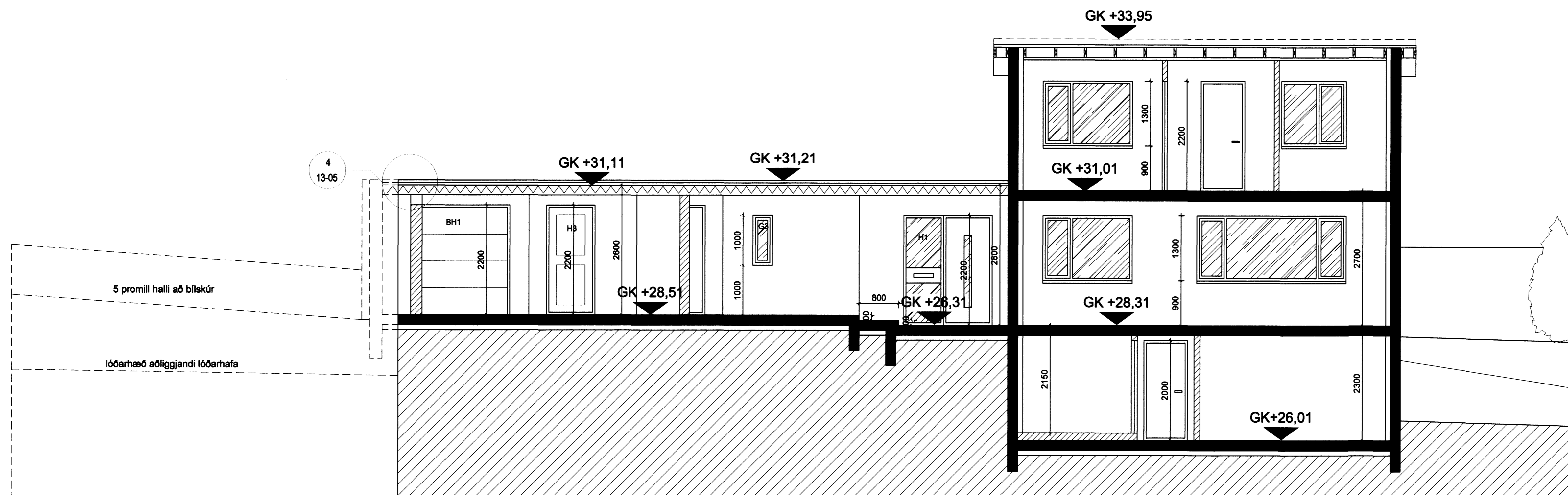
SNEIDING Y-Y 1:50
