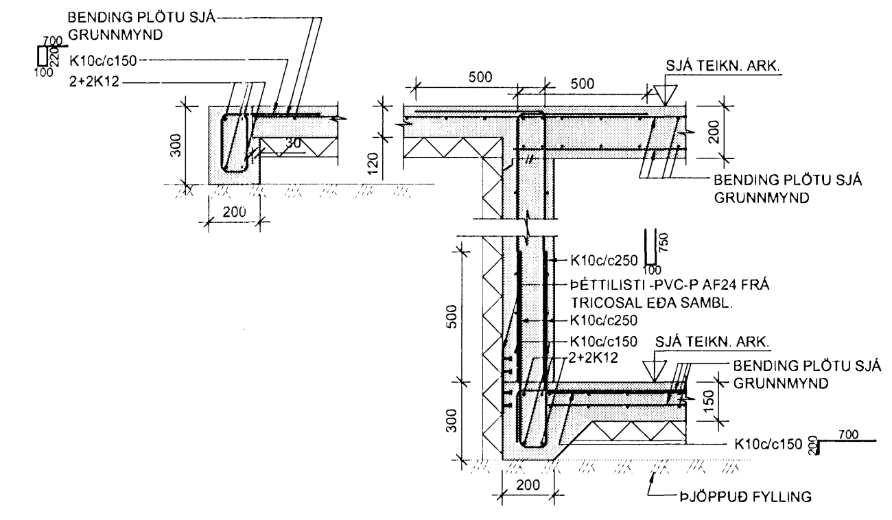
8 SNID 1:20
