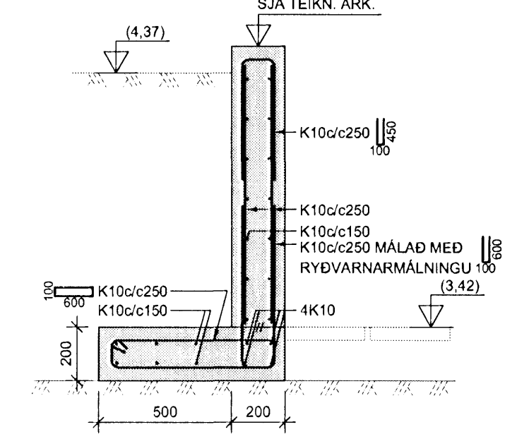
16 SNID 1:20
