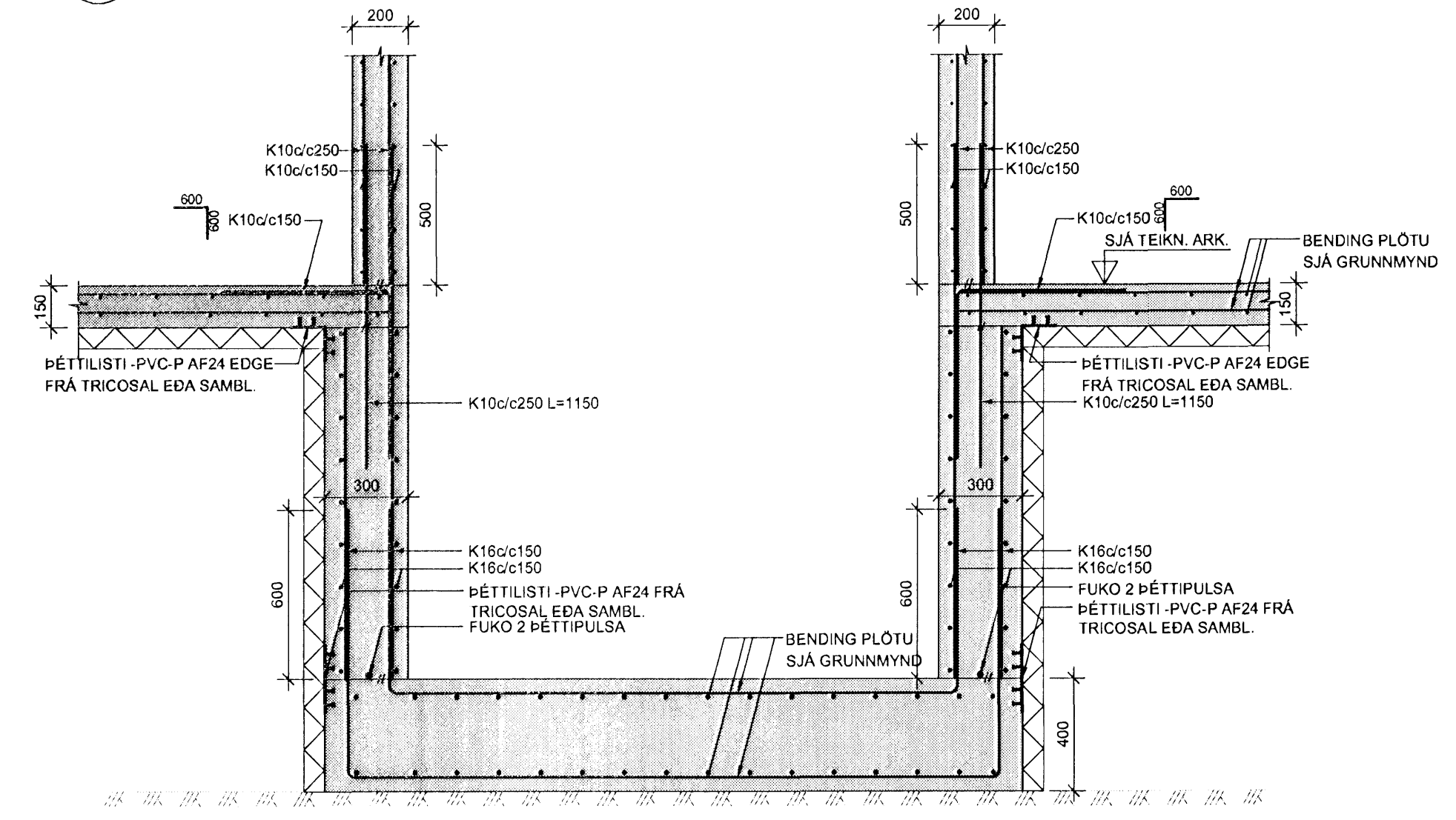
14 SNID 1:20
