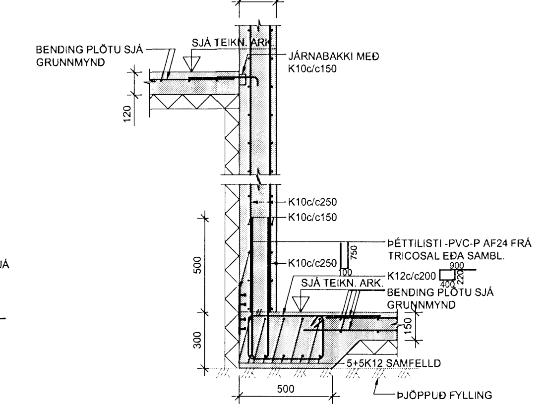
9 SNID 1:20
