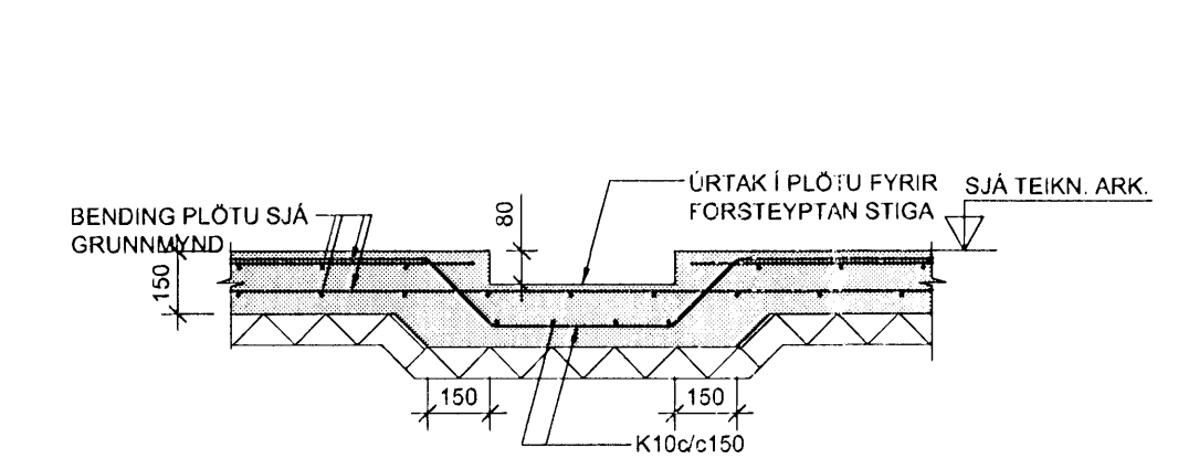
15 SNID 1:20
