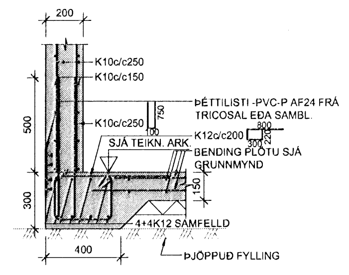
1 SNID 1:20
