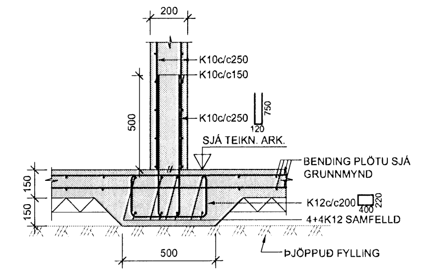
3 SNID 1:20
