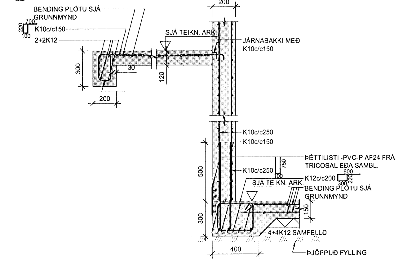
14 SNID 1:20
