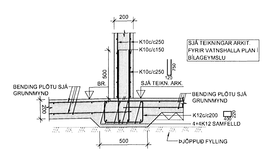
9 SNID 1:20
