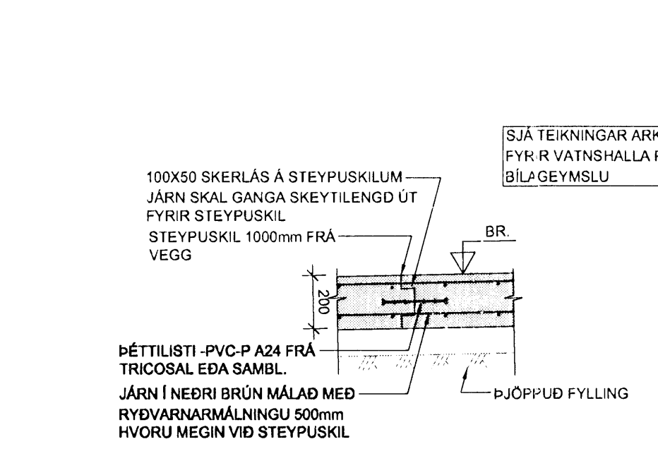
12 SNID 1:20
