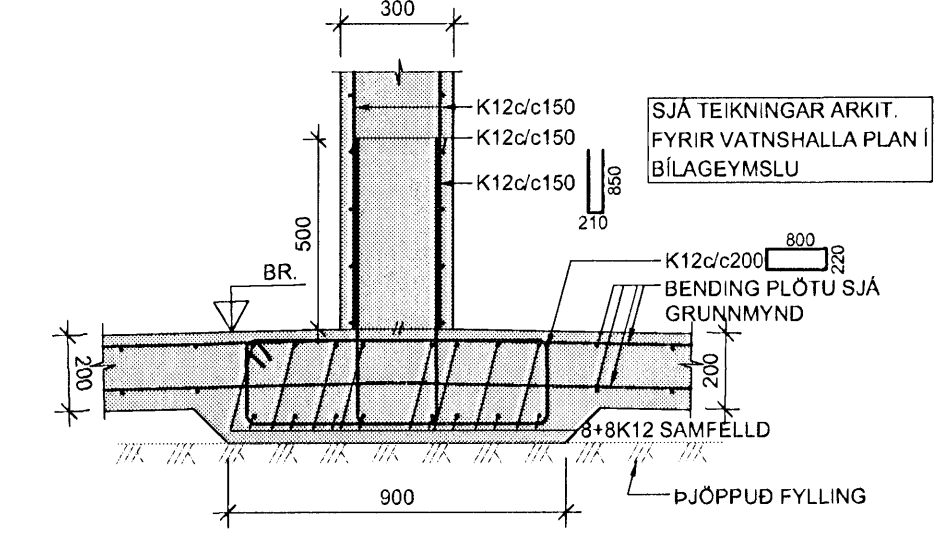
7 SNID 1:20
