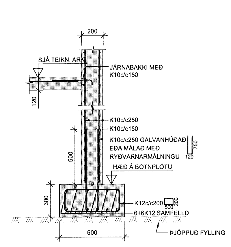
11 SNID 1:20
