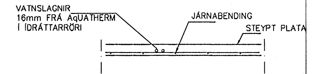
LAGNIR, SNID, 1:20
