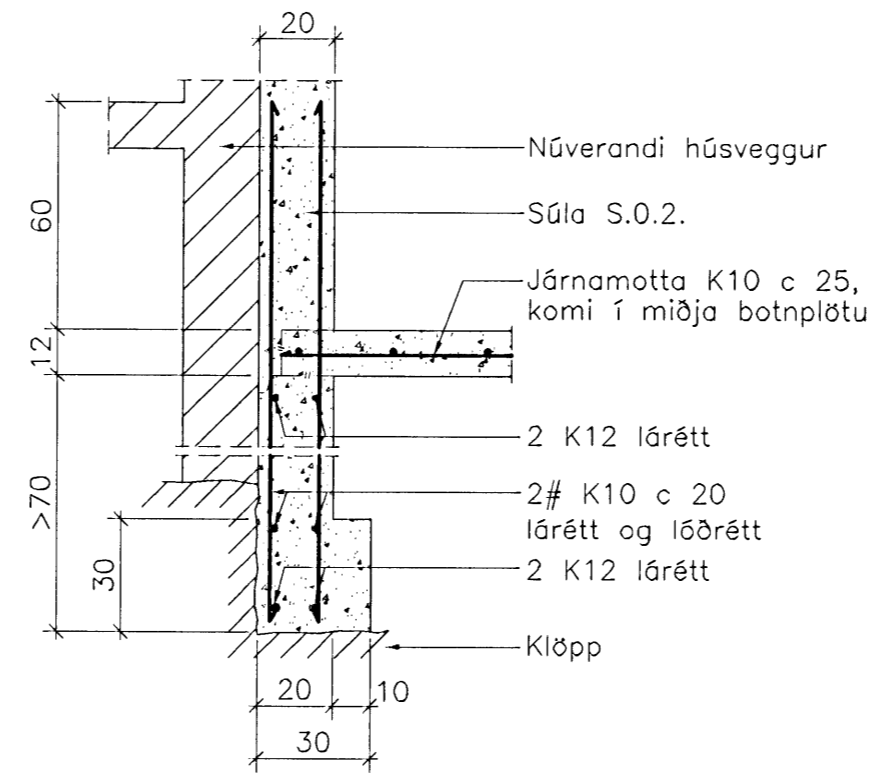
SNID C-C 1:20
