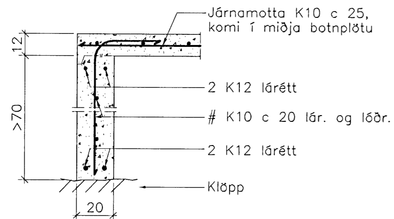
SNID E-E 1:20
