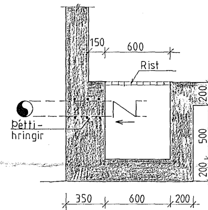
SNID C - C 1:20
