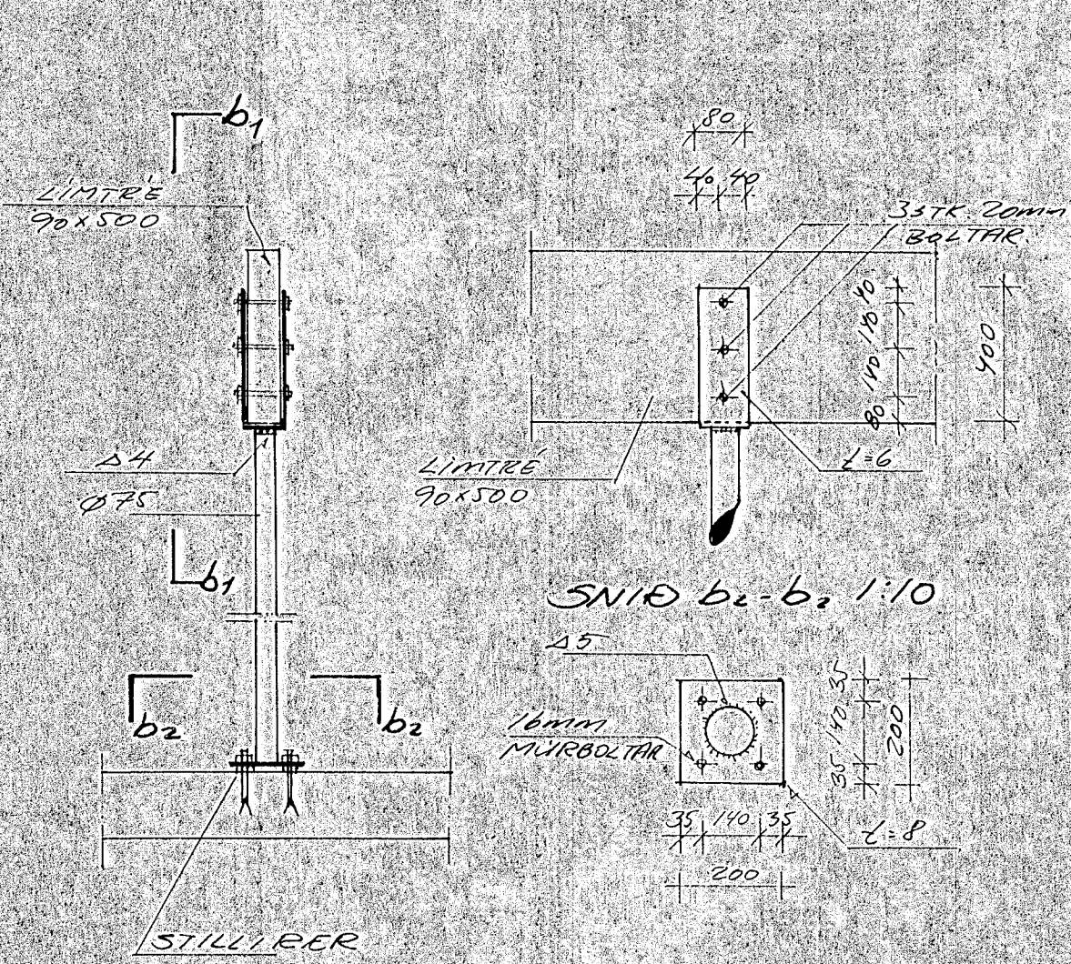
SNID B1-B1 1:20
