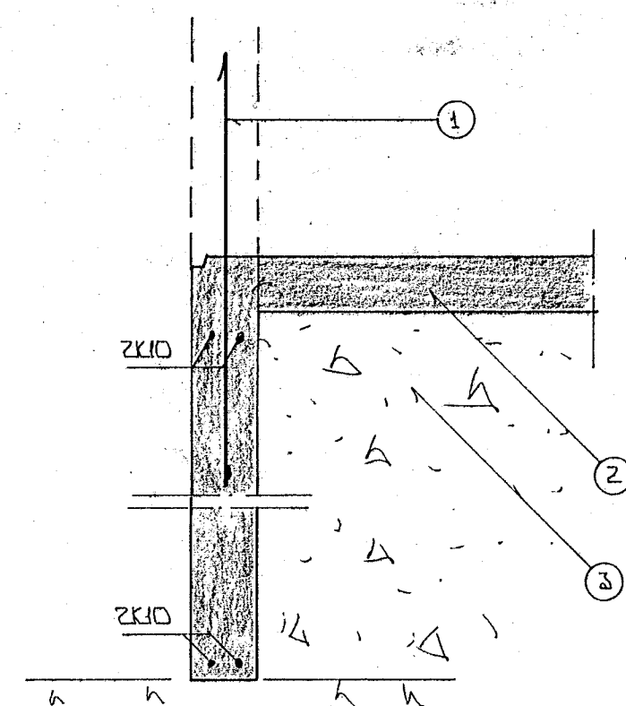
SNID 3 1:20
