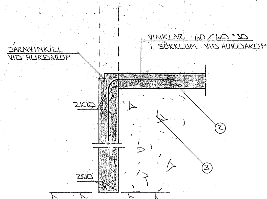
SNID 1 1:20
