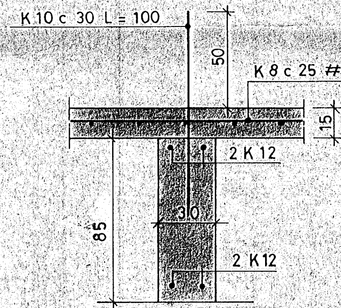
SNID C-C 1:20
