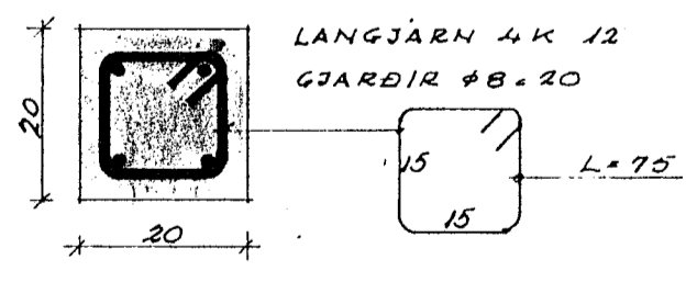
STODIR MILLI GLUGGA -1:10-
