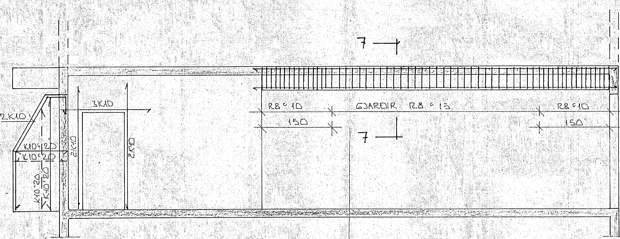
SNID 5 1:50 1-03
