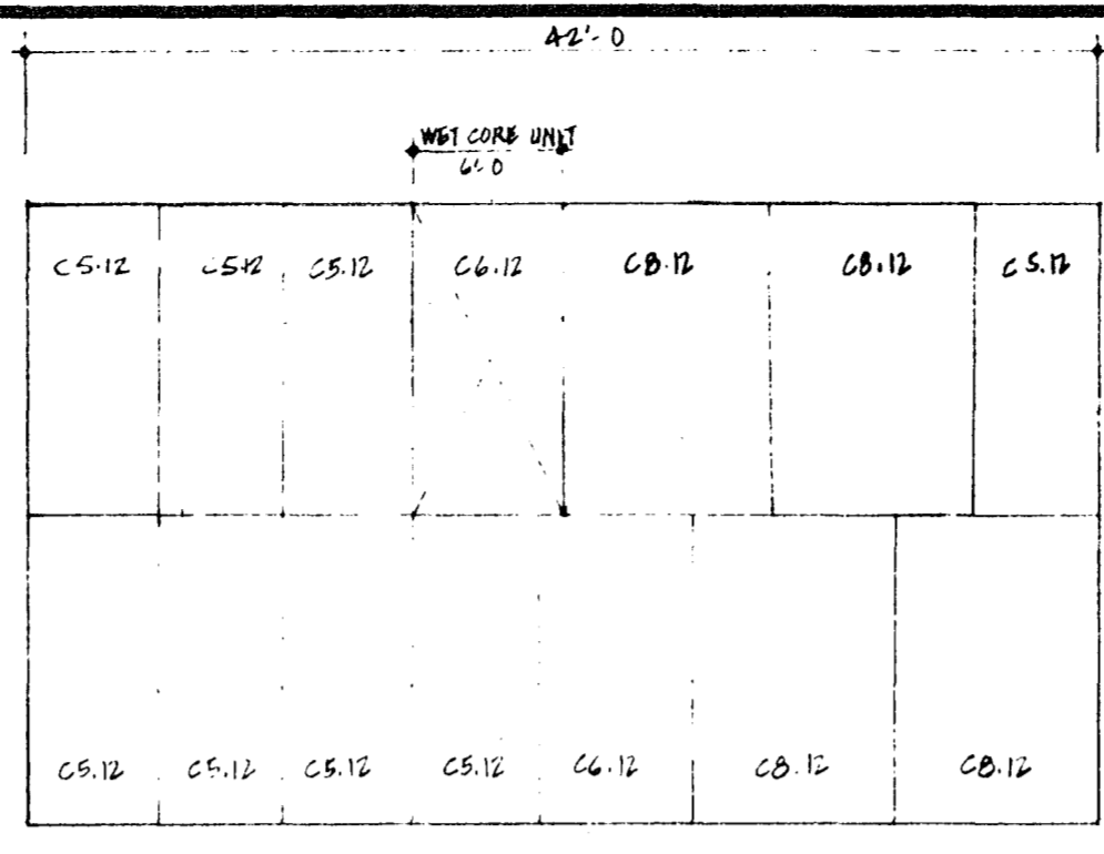
CEILING PANEL LAYOUT
