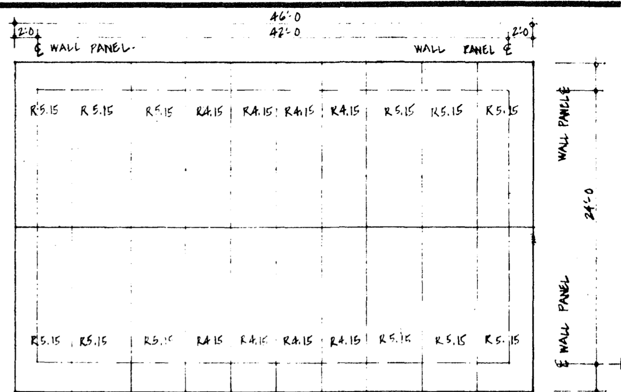
ROOF PANEL LAYOUT
