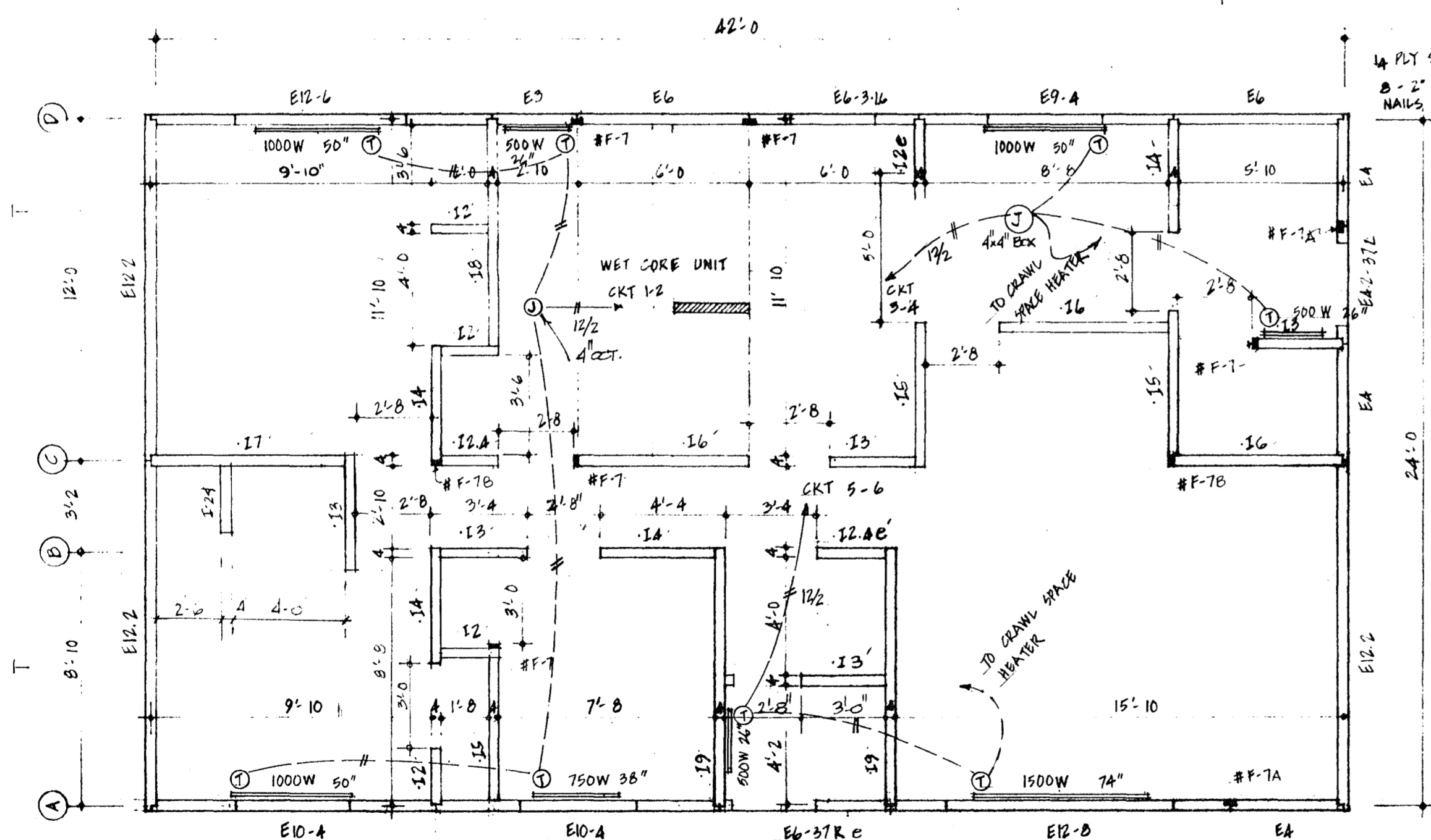
WALL PANEL LAYOUT (FLOOR PLAN)
