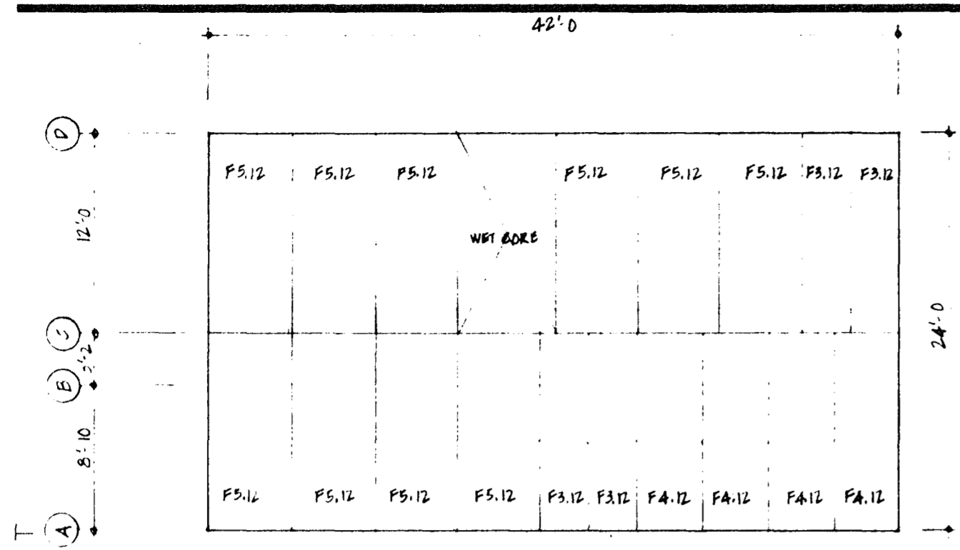
FLOOR PANEL LAYOUT
