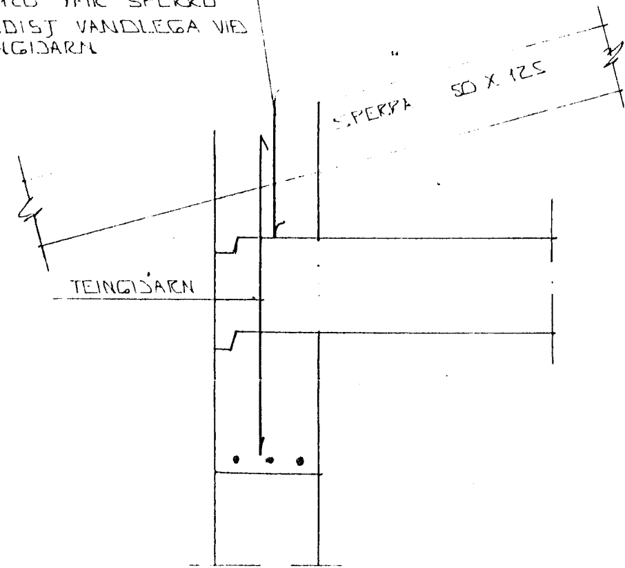
SNID 1 \times 1:10
