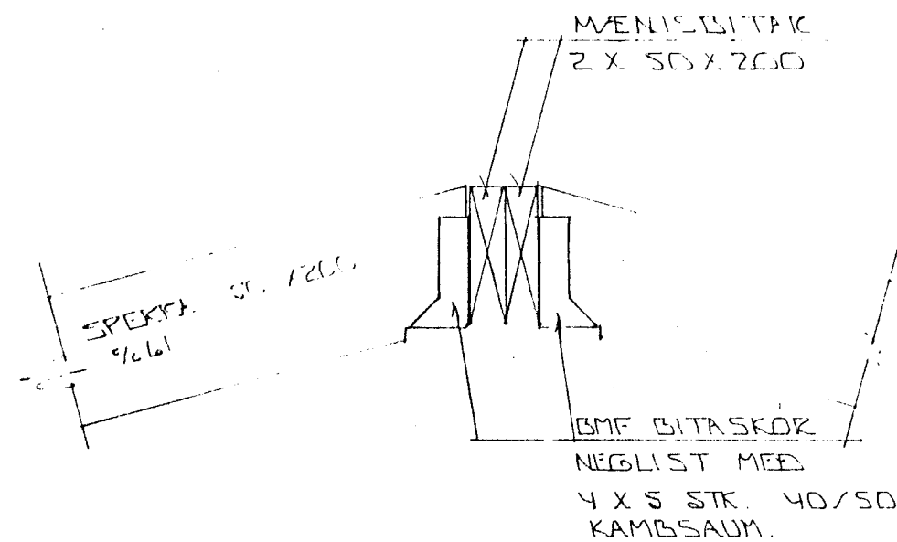
SNID 4 \times 1:10
