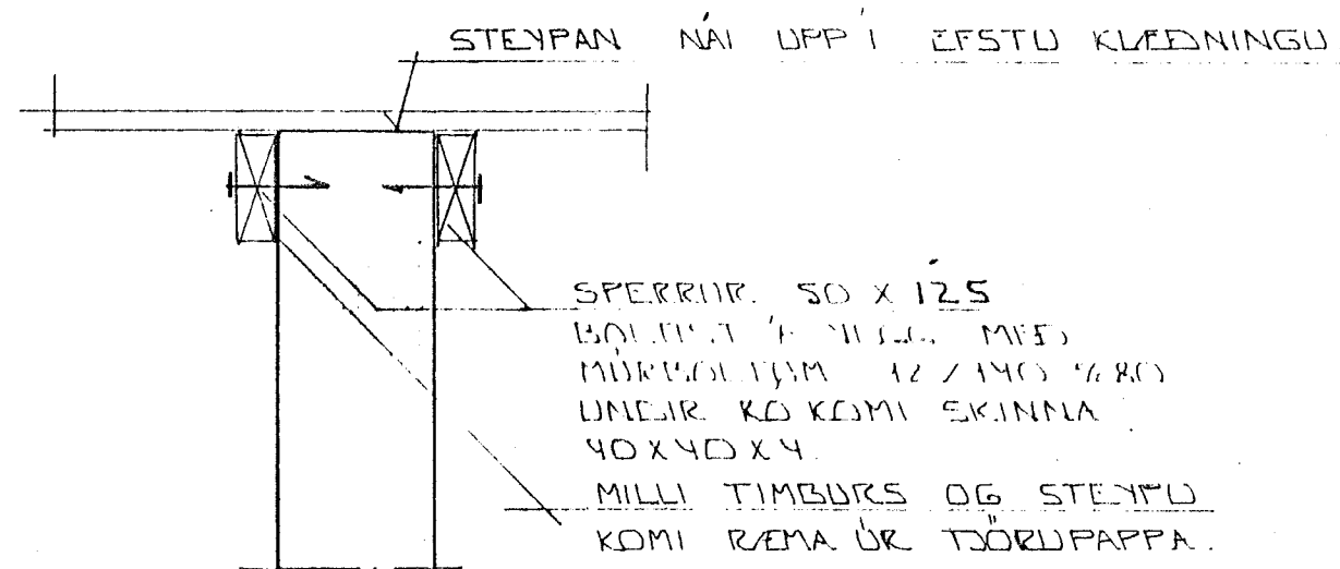
SNID 5 \times 1:10
