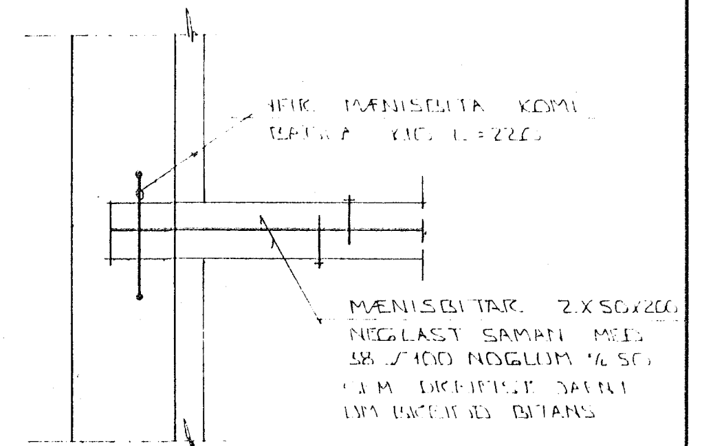
SNID 6 \times 1:10
