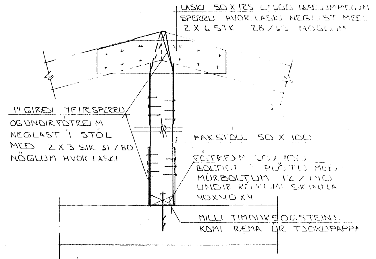
SNID 3 \times 1:10
