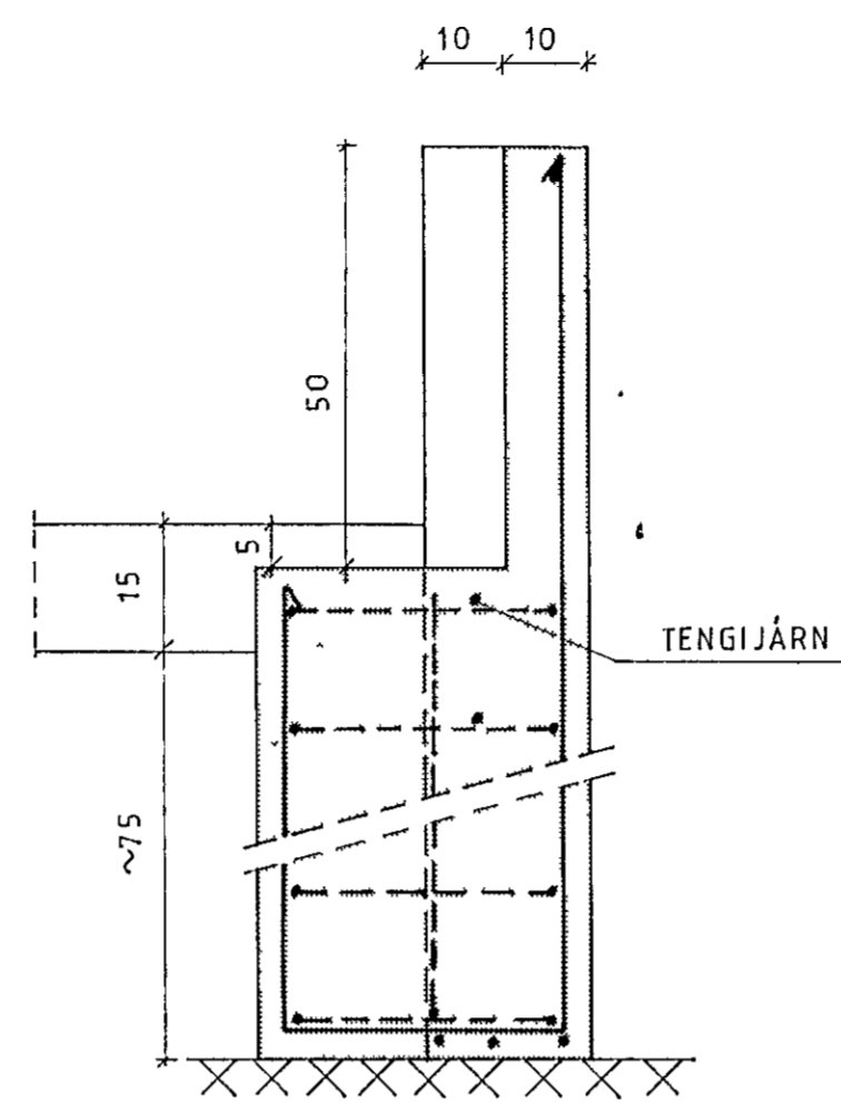
STOPULL B
