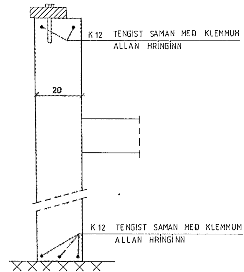
SNID C
