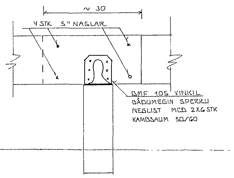
SNID F - F ~ 1:10
