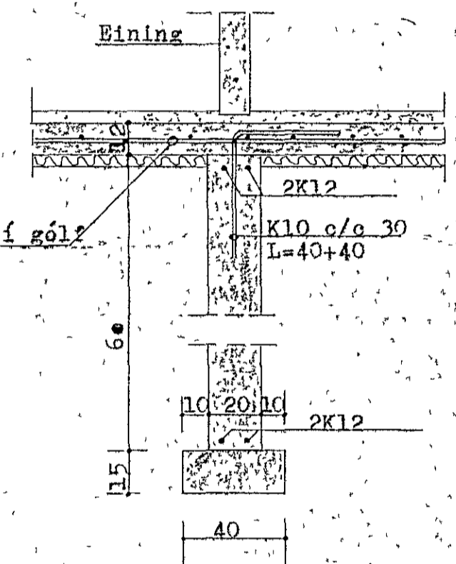
SNÍÐ B-B M: 1:20
