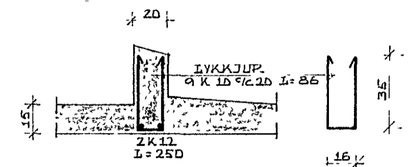
SNID C-C 1:20
