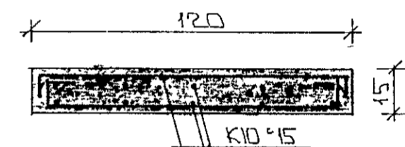
SNID 5-5-1-20
