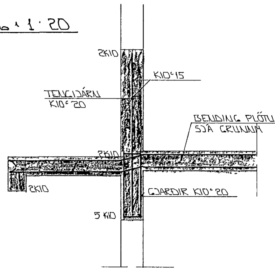
SNID 4-4-1-20
