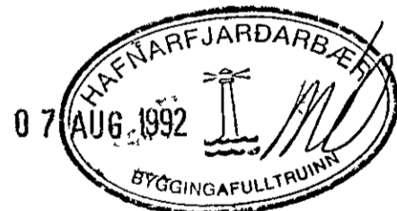
SNID 5-5-1-20
