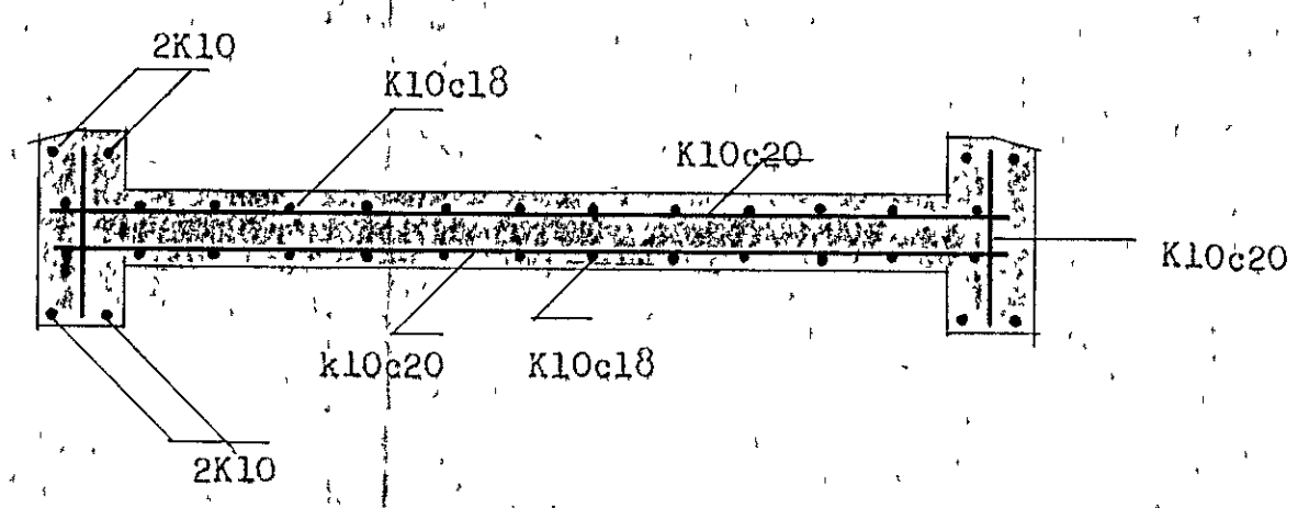
SNID E-E 1:20
