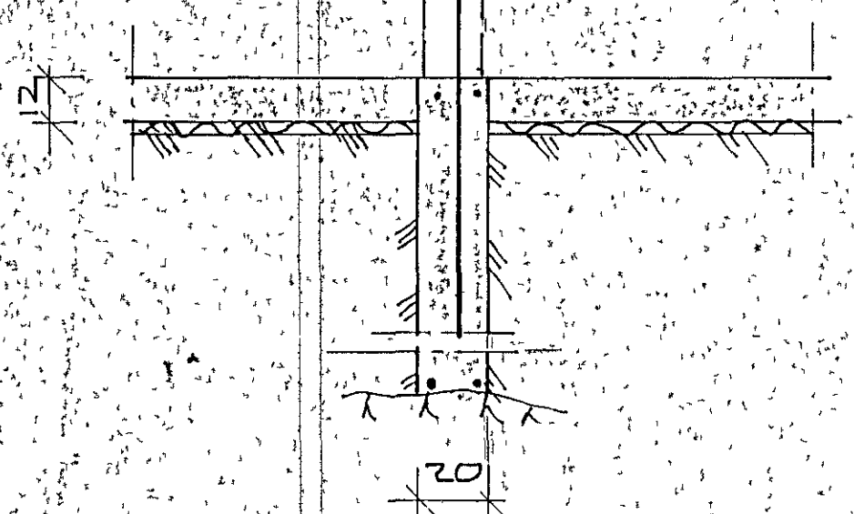
SNID J-J
