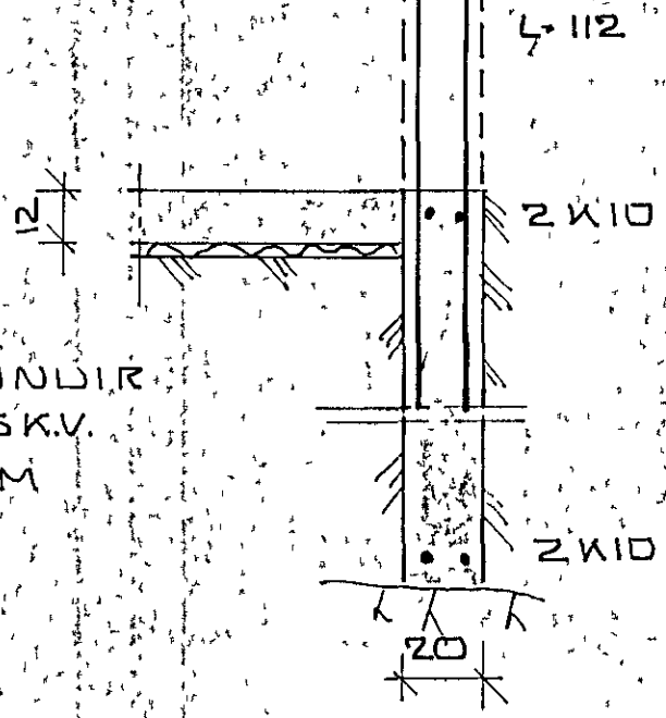
SNID E-E
