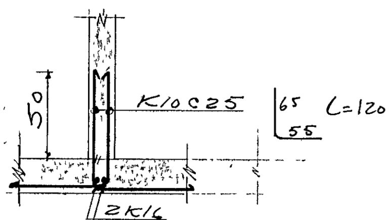
SNID C-C 1:20
