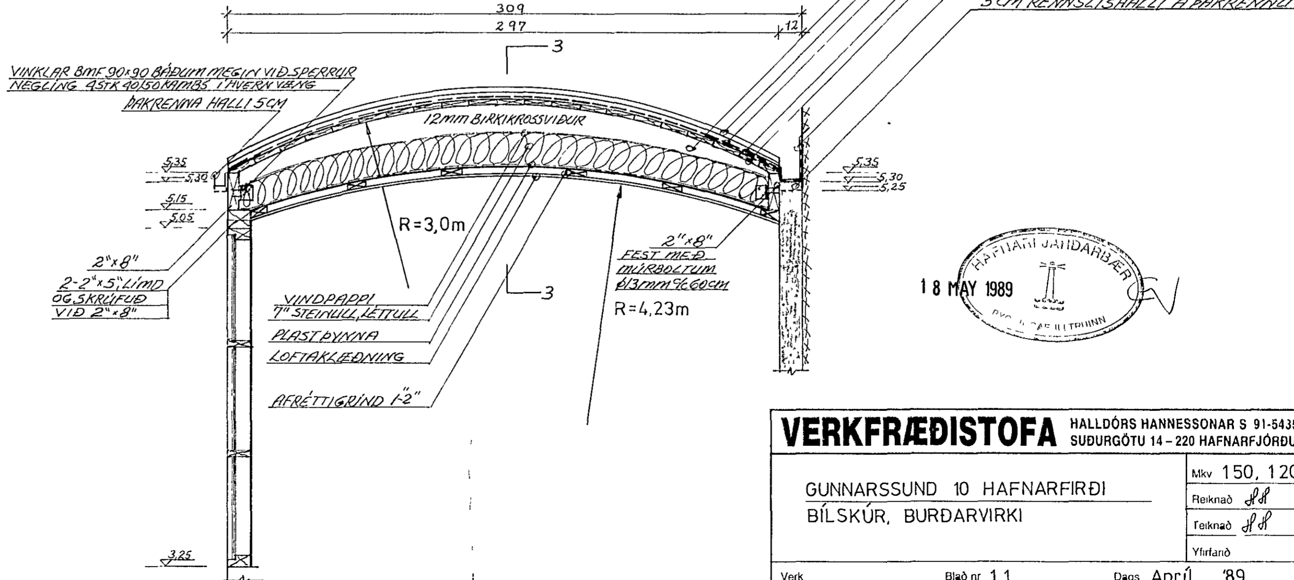
SNID 2-2 1:20
