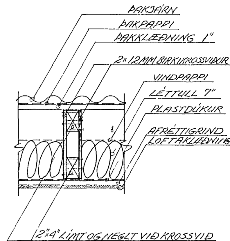
SNID 3-3 1:10
