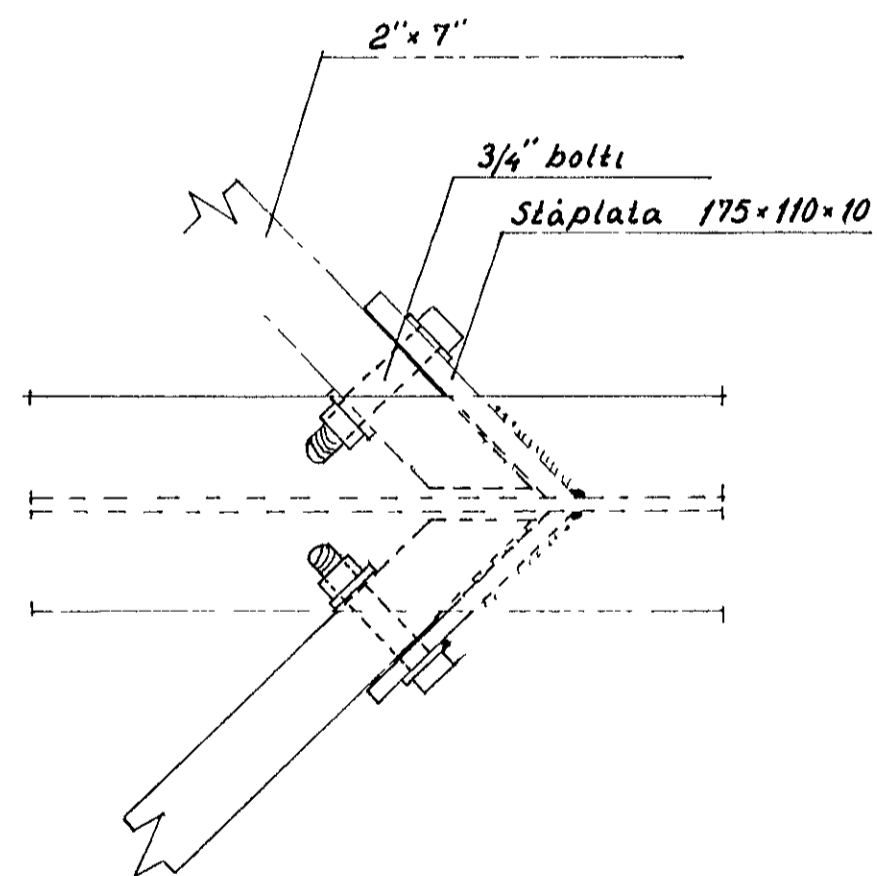
"A" M 1:5
