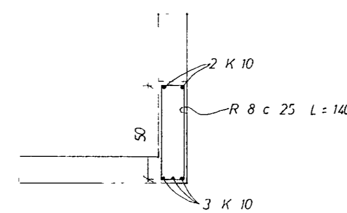
SNID B 1:20
