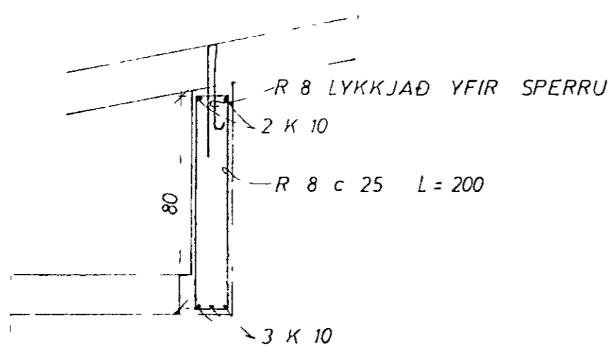
SNID A 1:20
