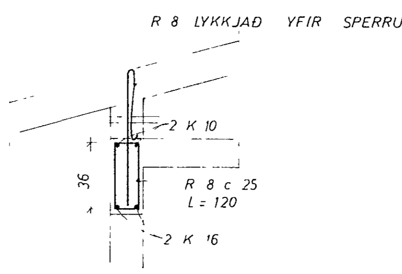
SNID C 1:20
